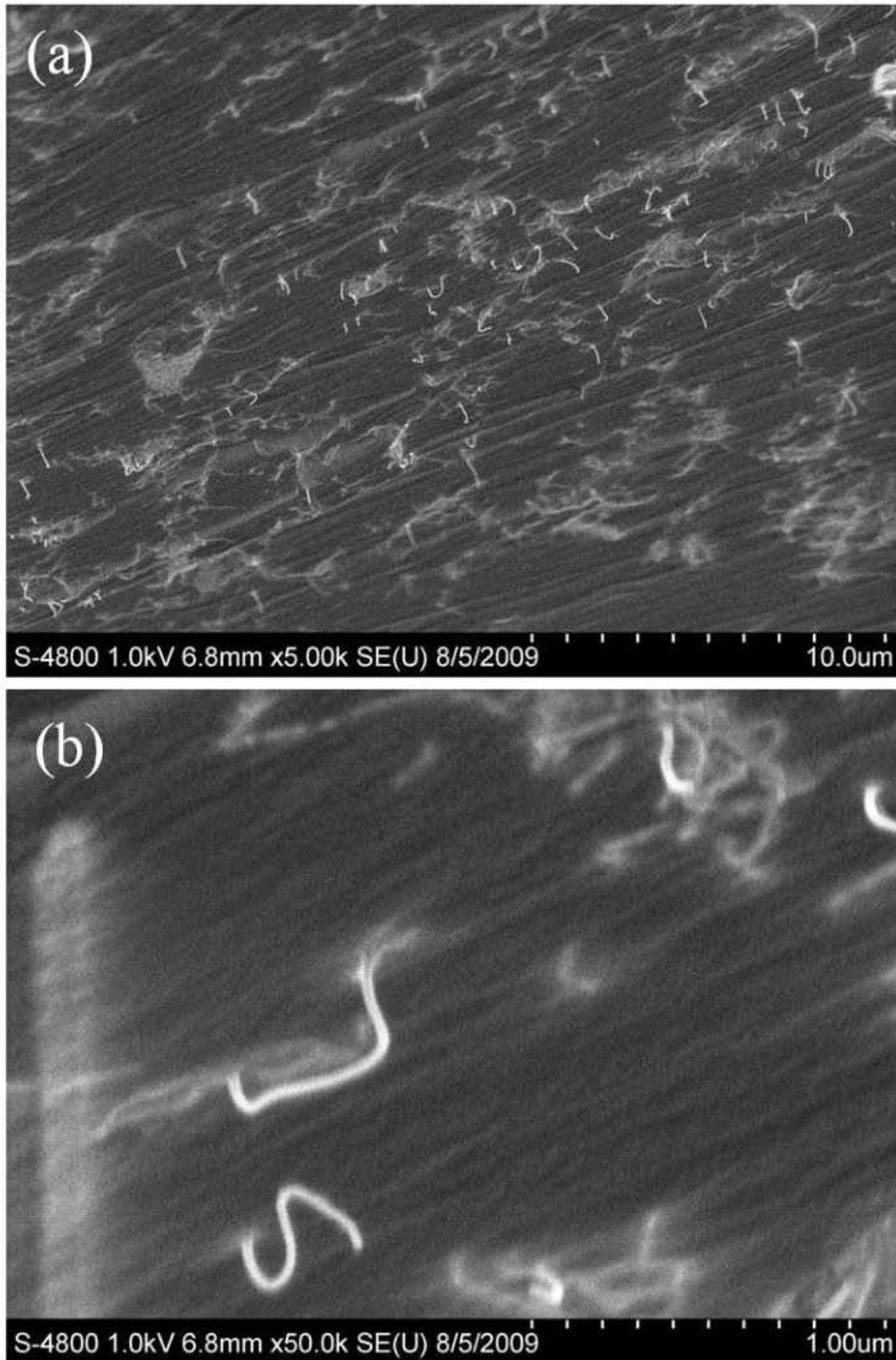
Figure 20: Secondary electron micrographs of 1.00 wt% SWCNT composite at: (a) 5kx and (b) 50kx magnification.
